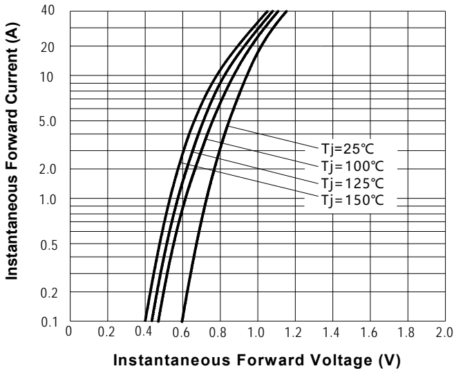
FIG3: Forward Voltage
