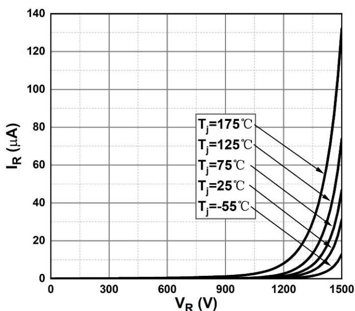
Figure 2. Reverse Characteristics
